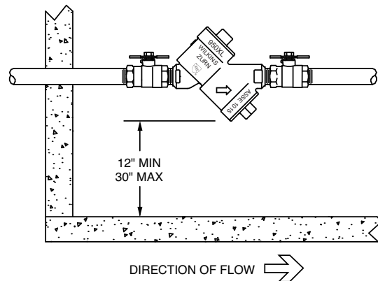
INDOOR INSTALLATION
