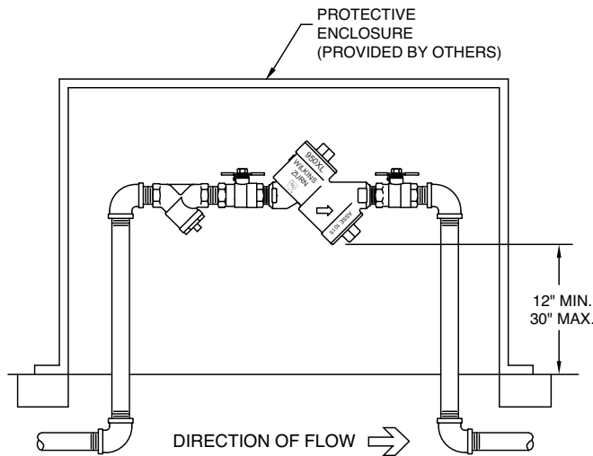
OUTDOOR INSTALLATION
